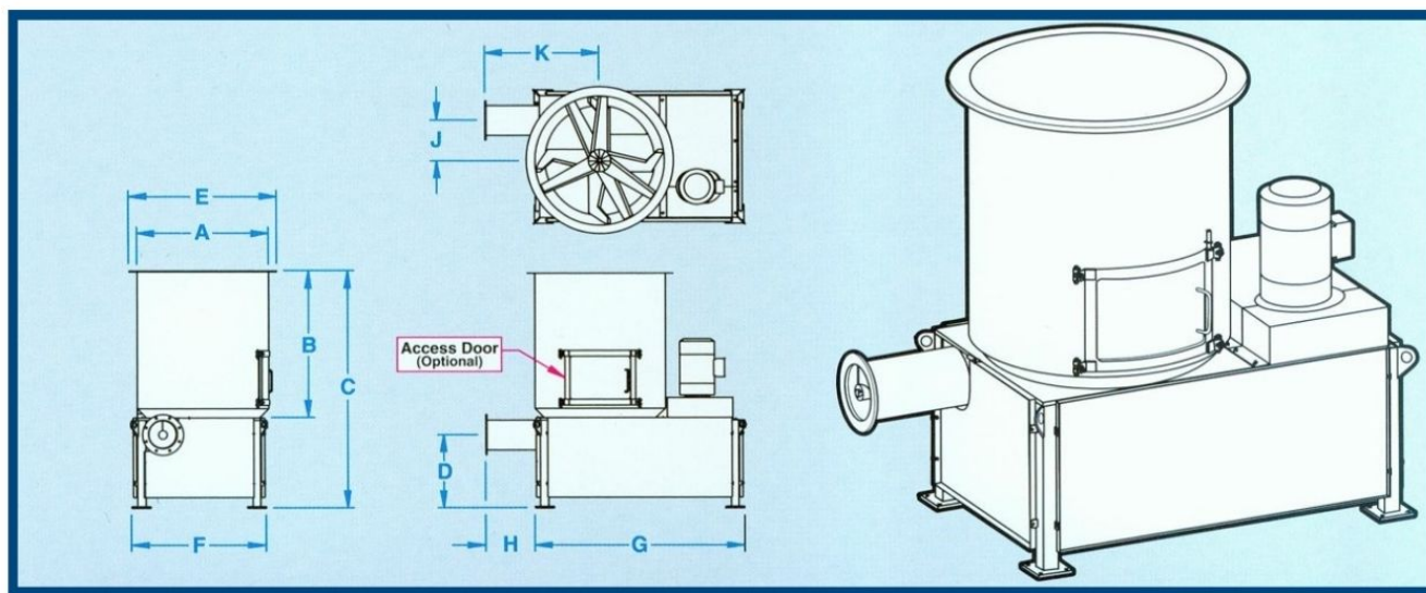
Cake Feeder Dimension Chart
