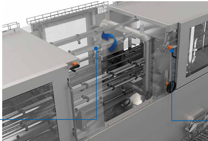
Quick-release fastening jetting pipes for easy installation and dismantling
