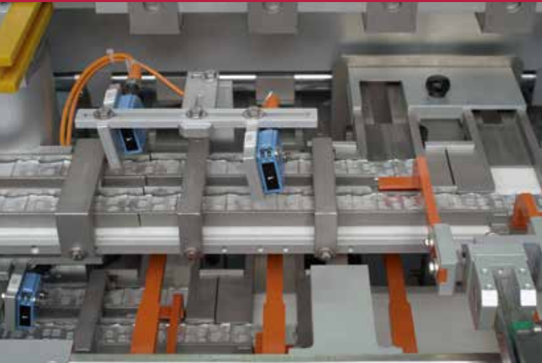
Product infeed
